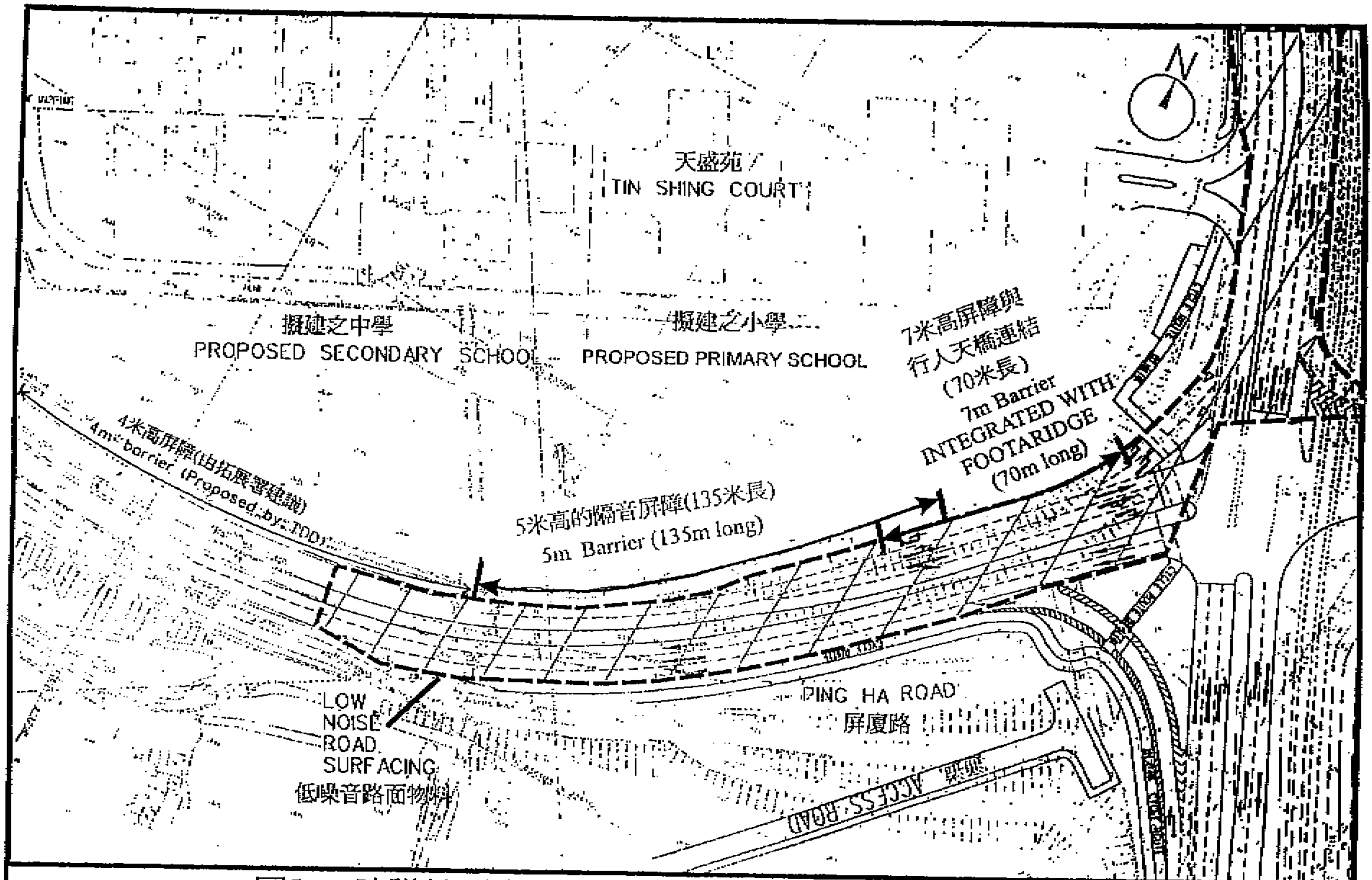
圖5.1 - 建議於天水圍，屏廈路興建之道路交通噪音直接緩減設施 FIGURE 5.1 - Proposed Direct Road Traffic Noise Mitigation Measures on Ping Ha Road, Tin Shui Wai
